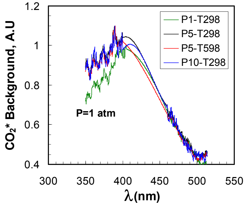
Figure 5.11. Spectral shape of the CO 2 * continuum in methane flames at various pressure conditions at \phi=0.75 .
