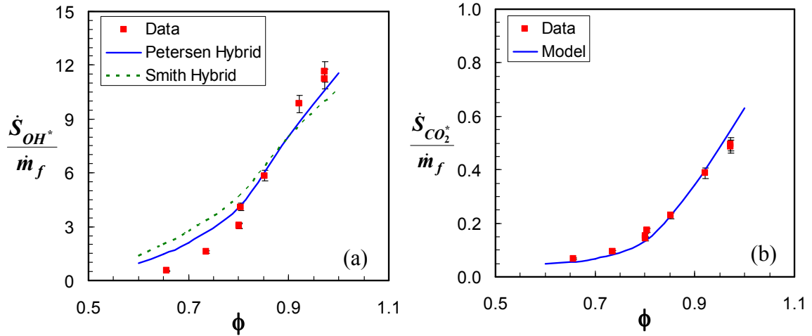
Figure 5.8. OH^* mechanism validation in methane flames at elevated pressure conditions: (a) normalized OH^* emission and (b) CO_2^* emission for flames at 10 atm and 300 K reactants.
