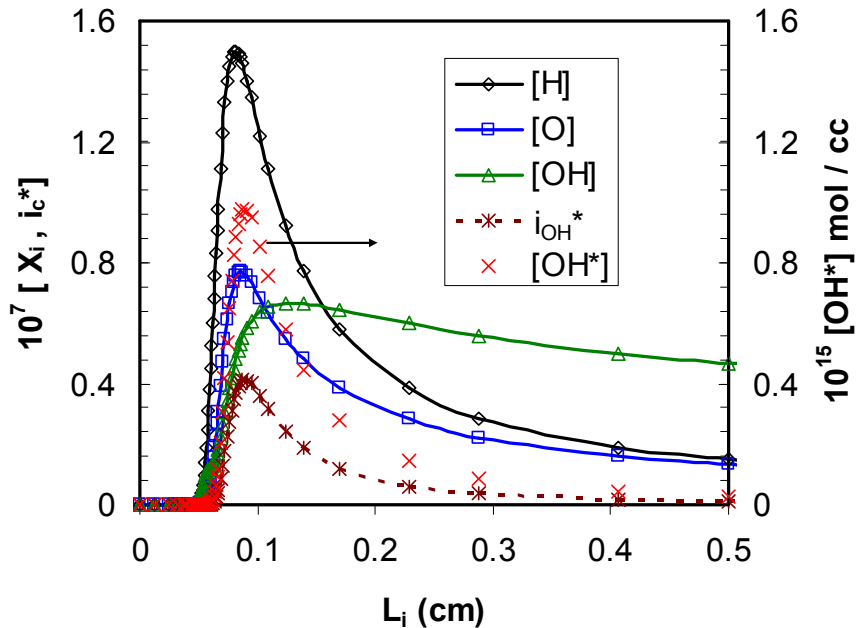
Figure 3.8. Sample CHEMKIN output for stoichiometric \text{H}_2:\text{CO}=50:50 syngas-air mixture at atmospheric ( P=1\text{atm} ) and non-preheated ( T=298\text{K} ) conditions. [\text{X}_i] ( \text{mol cm}^{-3} ) denotes species concentrations and i_{\text{OH}^*} ( \text{mol cm}^{-3} \text{s}^{-1} ) represents the volumetric photon emission rate for \text{OH}^* .
