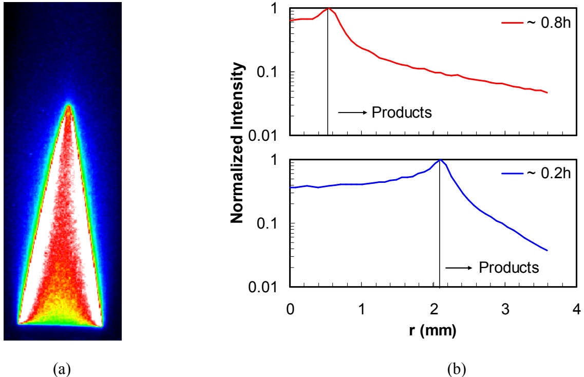
(a) (b) Figure 4.6. Chemiluminescence image analysis for a H_2:CO=50:50 flame at 10 atm, 598 K and \phi=0.9 . (a) Raw image (burner diameter is 6 mm) and b) radial (line-of-sight integrated) intensity profiles at 20% and 80% of the flame height.
