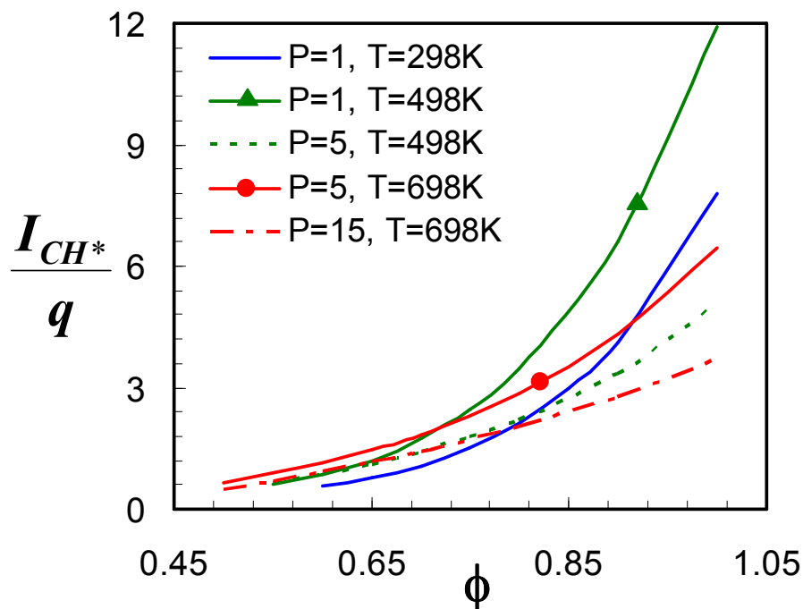
Figure 6.10. CH* chemiluminescence in methane at various pressure and preheat conditions.
