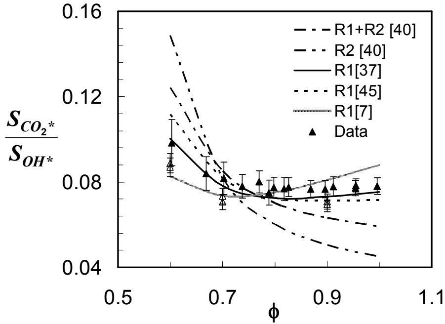
Figure 4.2. OH* mechanism validation: chemiluminescence intensity ratio predictions and experimental data in H_2:CO=50:50 syngas mixture. Simple tube burner (closed symbols); contour burner (open symbols).
